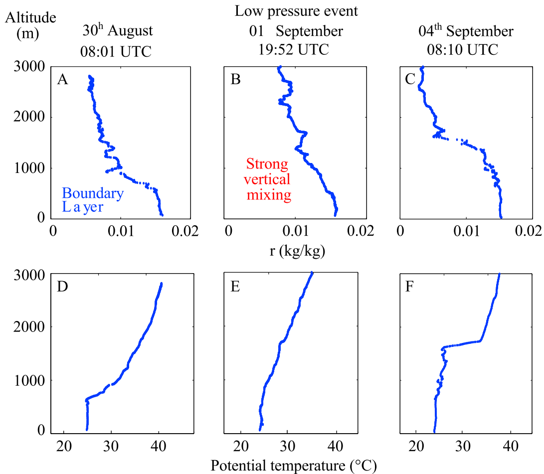
Figure 6. Vertical profiles of mixing ratio (a) before, (b) during, and (c) after the passage of the low-pressure event. Vertical profiles of potential temperature (reference level at 1000 hPa) (d) before, (e) during, and (f) after the passage of the low-pressure. The stratification between the PBL and the lower atmosphere was weak during the low-pressure event.
