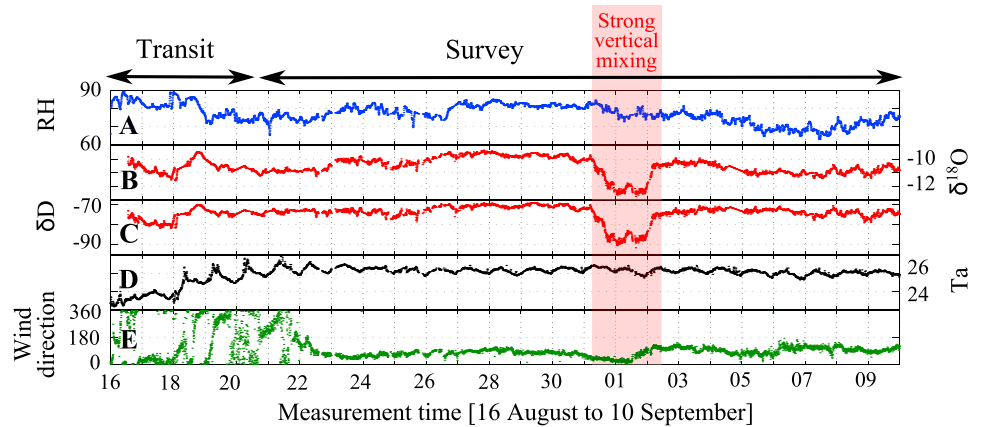
Figure 5. Evolution versus time of (a) relative humidity (%), (b) \delta^{18}\text{O} (‰), (c) \delta^2\text{H} (‰), (d) air temperature (degrees celsius), and (e) wind direction ( 0^\circ for northerly wind and 180^\circ for southerly wind) during the STRASSE cruise. The red shading period corresponds to important vertical mixing with the lower troposphere as diagnosed by radiosondages.
