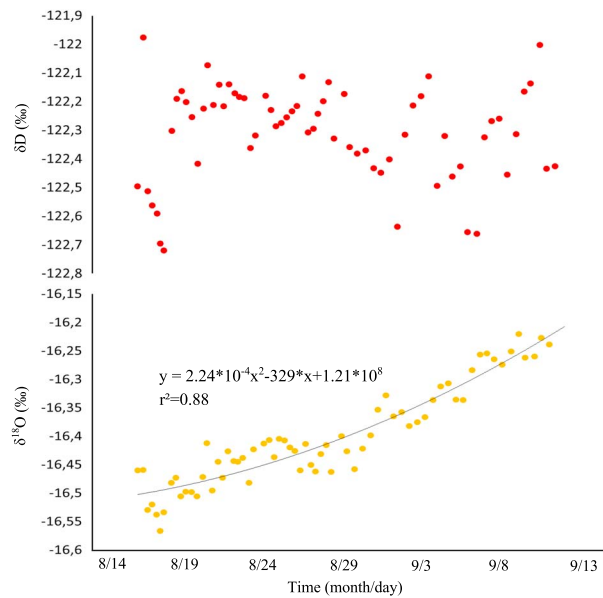
Figure 3. Drift of the Picarro L2130-I during the month of measurement. The accuracy is 0.05‰ for \delta^{18}\text{O} and 0.3‰ for \delta\text{D} . The drift for \delta^{18}\text{O} was 0.3‰. We chose not to correct the drift effect in \delta\text{D} measurements, because the accuracy of the \delta^2\text{H} measurement is comparable to the drift.
