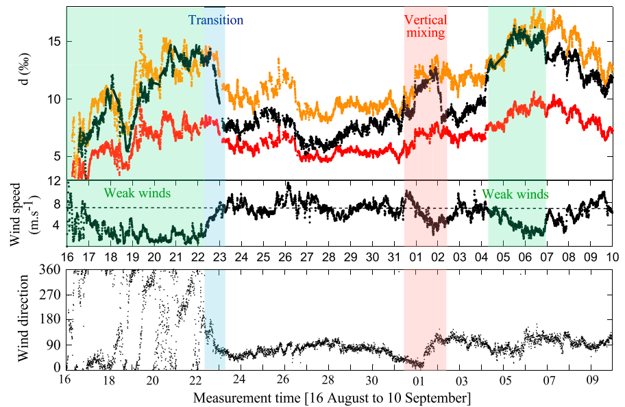
Figure 8. Variation of d-excess from 16 August to 10 September 2012. The black curve corresponds to measurements during the STRASSE cruise. The orange (red) curve is d-excess calculated with kinetic fractionation factor for smooth (rough) regime. The green shading is for the smooth regime and the blue shading is for a transition period. The red shading period corresponds to important vertical mixing with the lower troposphere. (middle) The wind speed corrected at 10 m. The dotted line corresponds to 7 \text{ m s}^{-1} , the transition between smooth and rough regime. (bottom) The wind direction.
