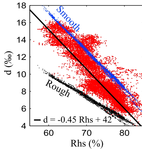
Figure 7. Correlations of d-excess in water vapor versus Rh s . The red points correspond to the measurements during the STRASSE cruise. The dark line represents a linear regression based on all the data ( d = -0.45 \text{ Rh}_s + 42 ). The blue (black) points are d-excess calculated from the closure equation for the smooth (rough) regime.
