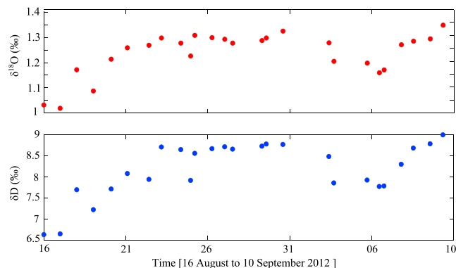
Figure 4. Isotopic composition of the 26 surface sea water samples during the cruise. The red and blue points are, respectively, measurements for \delta^{18}\text{O} and \delta\text{D} . The sampling depth is 3 m below the sea surface. All the samples were analyzed in laboratory LOCEAN with an accuracy of 0.05‰ for \delta^{18}\text{O} and 0.3‰ for \delta\text{D} .
