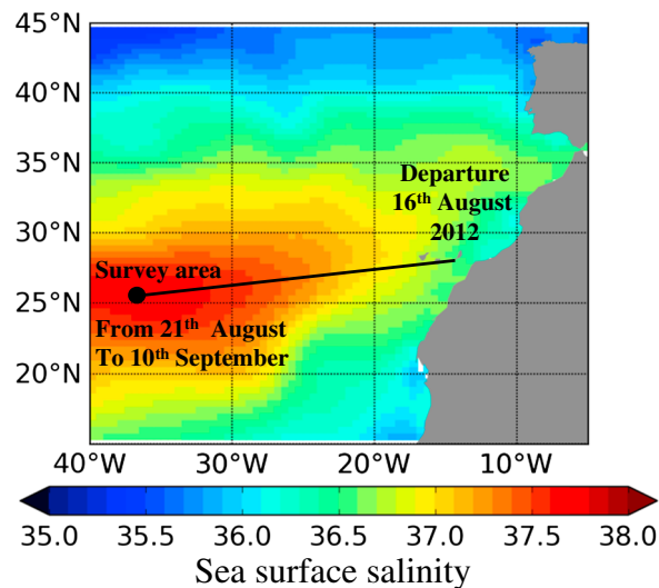
Figure 1. Trajectory of the ship during the STRASSE cruise. The ship left the Canary Islands on 16 August and arrived 5 days later in the survey area around 26°N, 35°W where it stayed 3 weeks. The survey area in the NE Atlantic corresponds to the region of salinity maximum (37.75‰) where evaporation exceeds largely precipitation in this season (the salinity map is from ISAS (In Situ Analysis System) objective analysis of Argo profile data for August 2012). The ISAS method is described in Gaillard et al. [2009].
