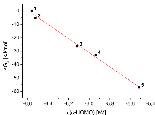
Fig. 4 Correlation \epsilon(\sigma\text{-HOMO}) [eV] and \Delta G_R [kJ/mol]
