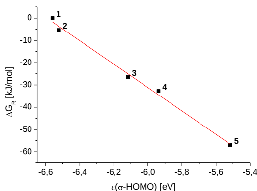
Fig. 4 Correlation \varepsilon(\sigma\text{-HOMO}) [eV] and \Delta G_R [kJ/mol]
