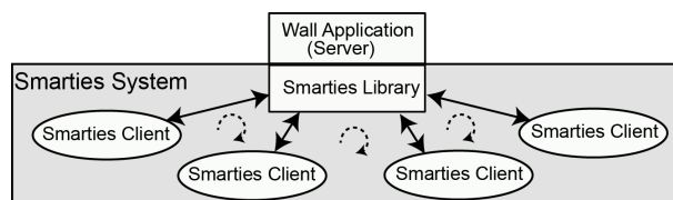
Figure 2. Basic Architecture. Rounded arrows indicate that the mobile clients communicate via the library, e.g. if a puck is moved in a client, this information is sent to the library that (i) transforms it into an event for the application developer; and (ii) sends it back to the other clients.
