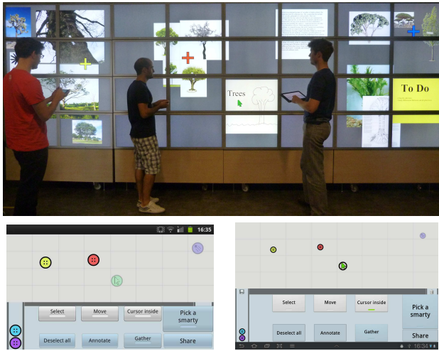
Figure 3. Object selection and grouping with three users. The interface running on a phone (left, middle user) and on a tablet (right, right user). Six state button widgets have been added by the application. The "Cursor Inside" action (device on the right) is attached to the active green puck, and acts as a mouse cursor confined inside a window.
