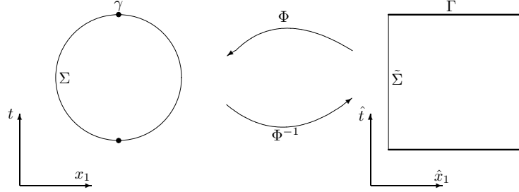
FIGURE 3.1. Change of variables transforming square into circle
