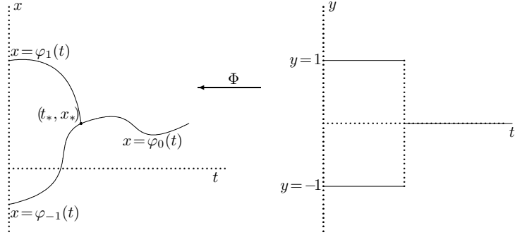
FIGURE 3.3. Case of two merging curves in \Sigma
