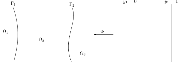
FIGURE 3.2. Case of several non-intersecting hypersurfaces in \Sigma
