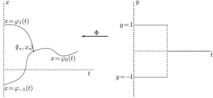
FIGURE 3.3. Case of two merging curves in \Sigma
