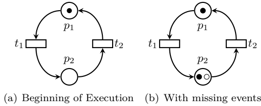
Figure 5. Token and tags
