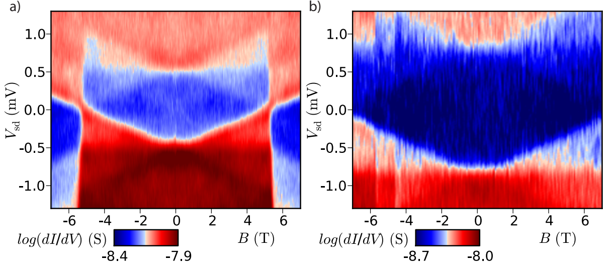
Fig.S. 2: Experimental differential conductance as a function of magnetic field for a fixed gate voltage V_g < V_g^D ( n_{C_{60}} = 1 ) for (a) J = -0.3 meV (second run) and (b) J = -0.4 meV (first run).
