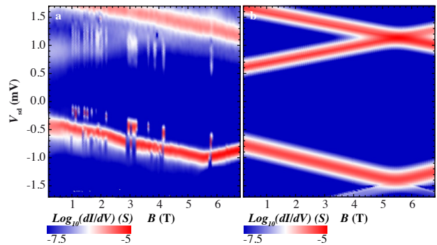
FIG. 3: Color scale plot of the differential conductance dI/dV as a function of bias voltage and magnetic field B . (a) shows experimental results while (b) shows numerical results in the regime where the ground state is n_{C_{60}} = 2 , with \epsilon_d = -3.1722 eV, U = 3.0 eV, J = -0.3 meV, C_g : C_R : C_L = 1 : 3.29 : 3.43 , and \Gamma_R/\Gamma_L \simeq 6.7 .
