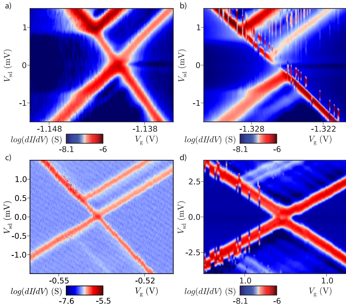
Fig.S. 1: Color scale plot of the differential conductance dI/dV as a function of bias voltage V_{sd} and gate voltage V_g : a) first run of measurements. b) second run of measurements. c) and d) other N@C 60 SMT's in the weak coupling regime.
