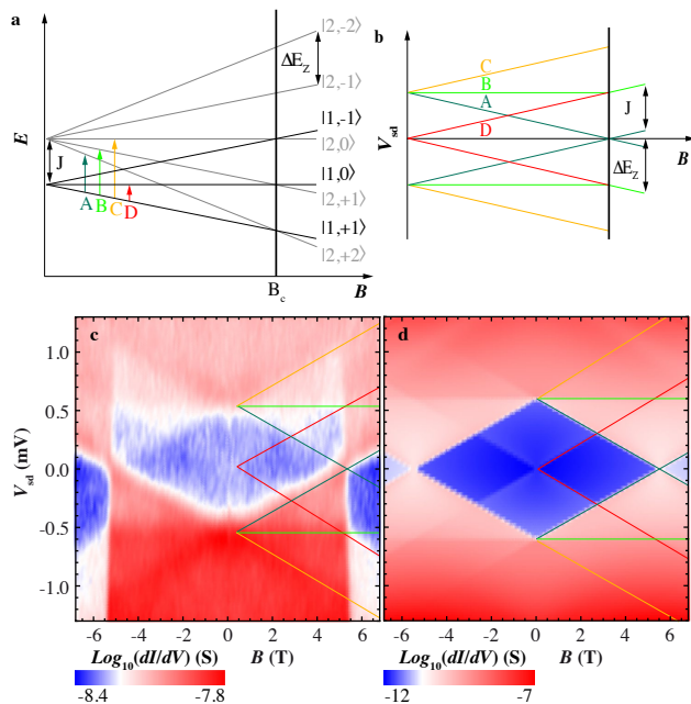
FIG. 4: (a) Zeeman diagram of the multiplets S = 1 and S = 2 for \text{N}@C_{60}^{1-} ( n_{C_{60}} = 1 ). (b) Schematic showing the expected cotunneling steps. (c) Experimental and (d) numerical results, with J = -0.3 \text{ meV} , of dI/dV for a fixed gate voltage V_g < V_g^D . Colored lines indicate the positions of the magnetic excitations illustrated in (a) and (b).
