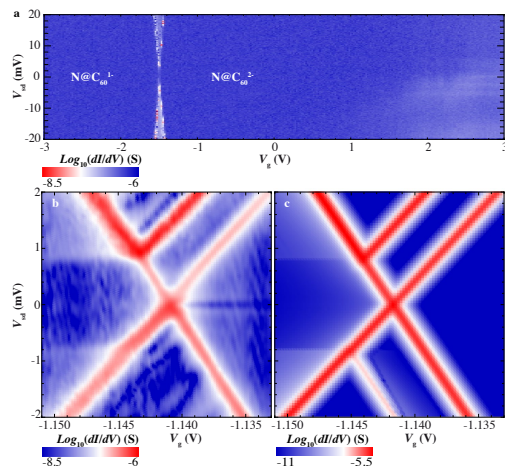
FIG. 2: Color scale plot of the differential conductance dI/dV as a function of bias voltage V_{sd} and gate voltage V_g (a) on the entire accessible V_g range and (b) in the vicinity of V_g^D . (c) Numerical results obtained from Eqs. (4) and (5) for \varepsilon_d = -3.1625 \text{ eV} , U = 3.0 \text{ eV} , J = -0.4 \text{ meV} , C_g : C_R : C_L = 1 : 3.09 : 2.96 , and \Gamma_R/\Gamma_L \simeq 10 .
