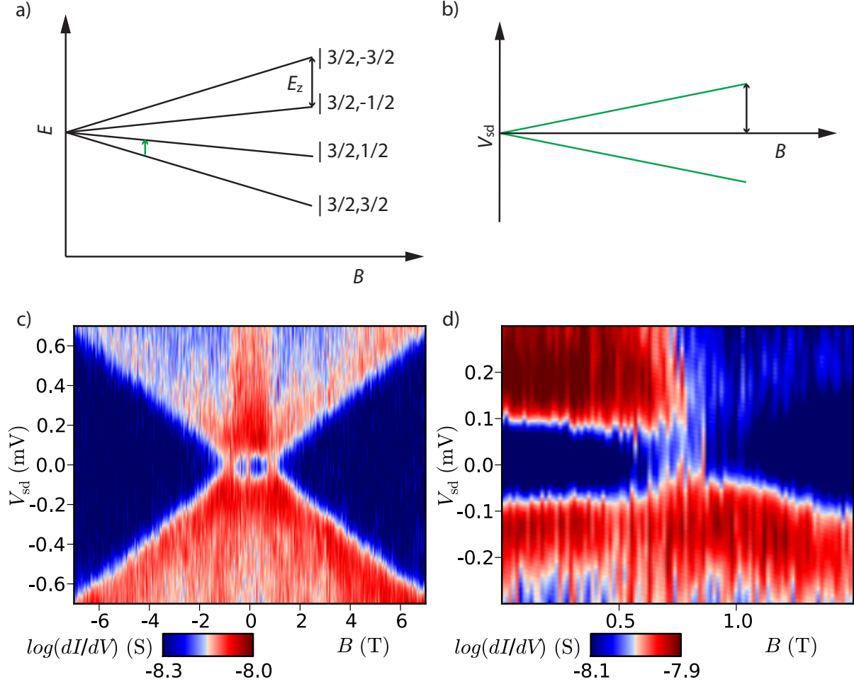
Fig.S. 3: (a) Zeeman diagram of the multiplet S = 3/2 for \text{N@C}_{60}^{2-} ( n_{\text{C}_{60}} = 2 ). (b) Schematic showing the expected cotunneling steps deduced from the Zeeman diagram. (c) and (d) dI/dV measurements as a function of magnetic field for a fixed gate voltage.
