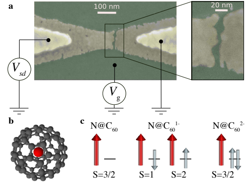
FIG. 1: (a) Colorized electron beam microscopy photograph of an SMT consisting of a gold nanowire over an Al/Al 2 O 3 gate after electromigration. (b) Schematic picture of N@C 60 . (c) Spins states of neutral and charged N@C 60 .
