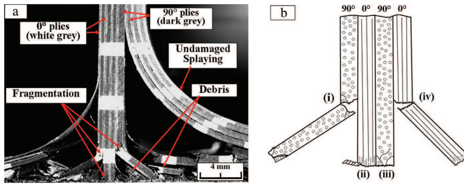
Fig. 2. (a) Major kinds of damage in mixed-mode crushing ( Note: white painted stripes are used to follow the plate displacement ) (b) fragmentation modes: (i) inside ply matrix cracking (ii) 0^\circ localized crushing (iii) 90^\circ localized crushing (iv) inside ply fiber breakage. (For interpretation of the references to colour in this figure legend, the reader is referred to the web version of this article.)
