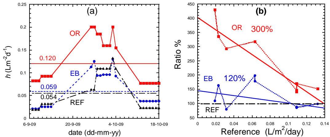
Figure 4. (a) Evolution of dew yields ( \text{Lm}^{-2}\text{day}^{-1} ) for the origami (OR, squares, full line), egg box (EB, short dashed line) and reference plane (REF, triangles, long dashed line) with mean values (horizontal lines). (b) Ratio R (%) of the condenser to the reference plane with respect to dew yields (OR, squares, full line), (EB, dashed line). The thick lines are 100% weighting of the data
