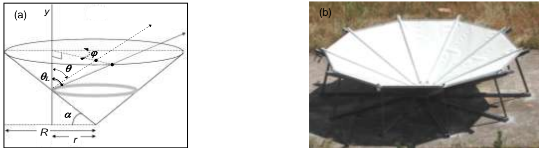
Figure 1. (a) Integration scheme for the funnel shape ( 0 < \theta < \theta_L , 0 < \varphi < 360^\circ and 0 < r < R ). (b) Photo of the funnel-shaped condenser ( 7.3 \text{ m}^2 surface area with 60^\circ cone angle, 30^\circ from horizontal). The internal surface of the experimental condenser is coated with OPUR ( www.opur.fr ) low density polyethylene foil insulated from below with 3 cm styrofoam.
