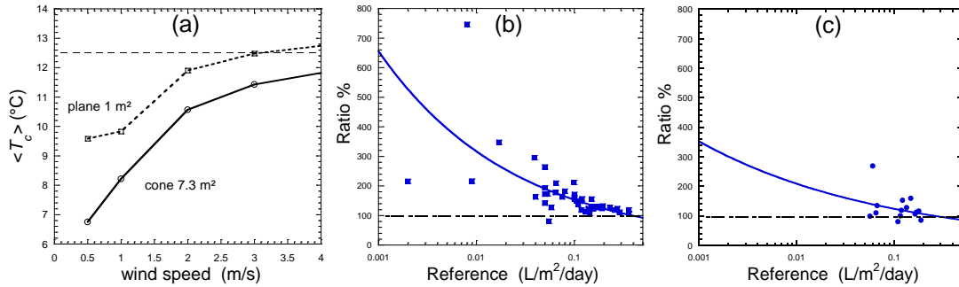
Figure 2. (a) Mean surface temperature \langle T_c \rangle with respect to wind speed. (b) Dew gain R of a 7.3\text{ m}^2 cone with respect to a 1\text{ m}^2 plane (semi-log plot; adapted from Clus et al., (2009)).(c) Id. for a pyramid collector, (adapted from Jacobs et al. (2008)).
