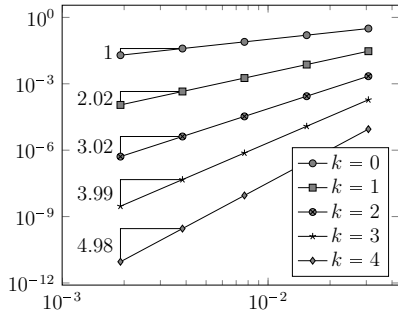
(a) Gradient error, triangular meshes
