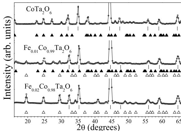
Figure 1. Neutron-diffraction spectra showing phase coexistence at x = 0.01 for the Fe_xCo_{1-x}Ta_2O_6 solid solution. The reflections indicated by solid triangles correspond to the magnetic phase described by propagation vectors (\pm 1/4, 1/4, 1/4) , while open triangles mark reflections of the phase with propagation vectors (\pm 1/4, 1/4, 0) . Vertical bars locate structural reflections of the P4_2/mnm space group. Continuous lines are Rietveld fittings to the data points.
