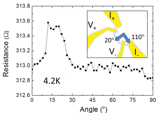
FIG. 1. Measurement of the resistance of the LSMO half ring as a function of the angular domain wall position. For directions between 10^\circ and 25^\circ (see inset), an increase of the resistance is observed, corresponding to a magnetic domain wall positioned between the two inner contacts of the wire.
