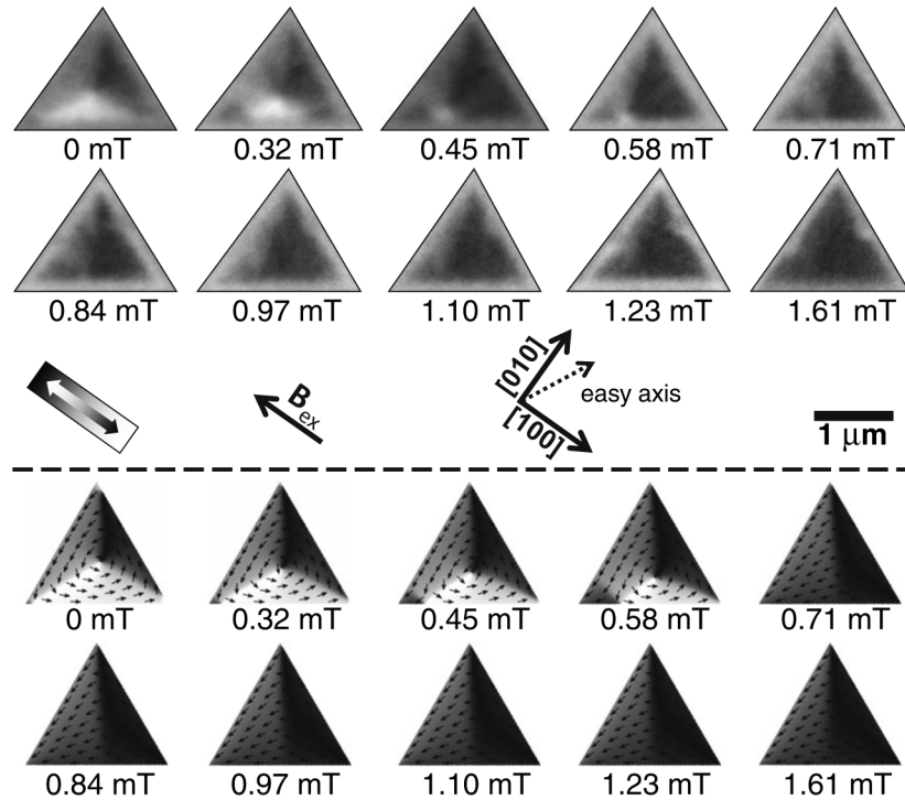
Figure 5. Field cycle of a 2 \mu\text{m} sized equilateral LSMO triangle of 15 \text{ nm} thickness. Top: XMCD-PEEM images; bottom: corresponding micromagnetic simulations.
