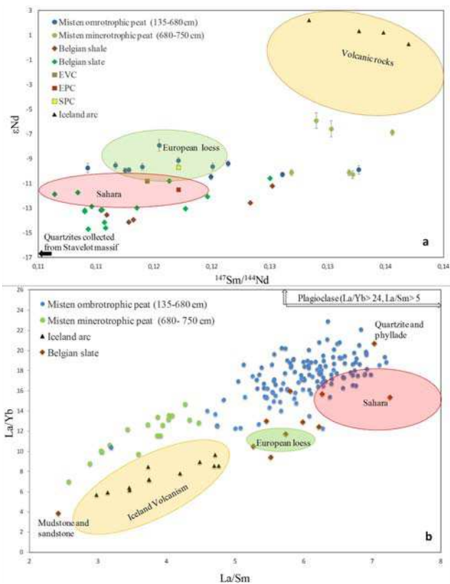
Fig. 8. (a) \epsilon Nd vs. ^{147}Sm/^{144}Nd diagram for Misten peat samples. (b) La/Yb vs. La/Sm diagram for Misten peat samples. Belgian shale data from André et al. (1986), Belgian slate data recorded from Brabant Massif (Linnemann et al., 2012), Saharan aerosol data from Abouchami et al. (1999), Variscan crust (EVC), Pan-African crust of northwestern Europe (EPC) and of the Scandinavian shield (SPC) from Fagel et al. (1999), Iceland arc from Handley et al. (2011) and European loess from Gallet et al. (1998).
