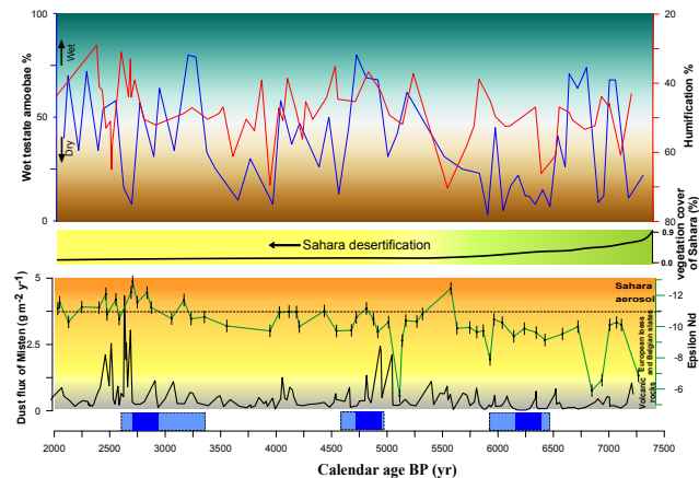
Fig. 9. Comparison of the Misten proxies (dust flux, \epsilon Nd , humification and testate amoebae). The testate amoebae were classified according to their affinity with wet conditions. The three dark blue bars show the cold events according to Wanner et al. (2011) and the three light blue bars show the uncertainty in the length of cold events. The Saharan desertification model is from Claussen et al. (1999).
