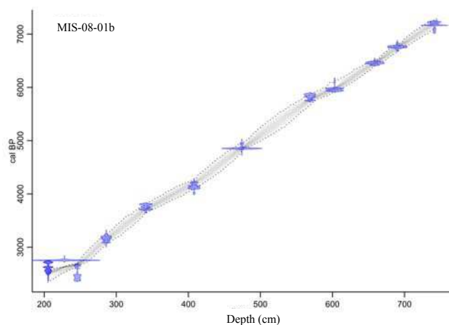
Fig. 2. Bacon age–depth model for the MIS-08-01b core. Grey scales indicate all likely age–depth models, and dotted lines indicate the 95 % confidence ranges.
