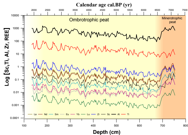
Fig. 4. Concentrations of Ti, Al, Sc, Zr and REE for the MIS-08-01b core. The yellow area corresponds to ombrotrophic peatland, the brown area to minerotrophic peat as defined by using Ca/Mg ratios, Sr concentration and testate amoebae assemblages.
