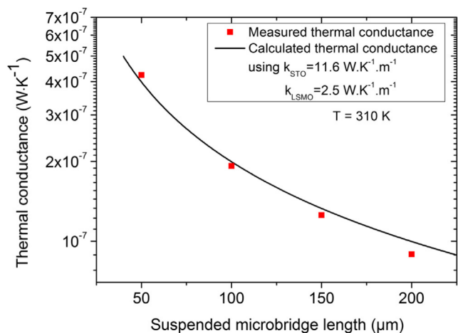
Fig. 4. Thermal conductance of 4 \mu\text{m} wide suspended LSMO microbridges versus microbridge length at 310 K.
