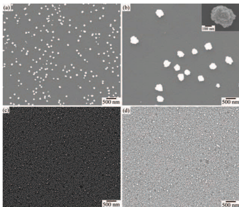
Fig. 3. FEG-SEM images of AuNPs-GC electrodes prepared from a deaerated 0.1 M NaNO 3 solution containing 0.25 mM HAuCl 4 by CPE at 0.7 V for (a) 10 s and (b) 1800 s and at -0.3 V for (c) 10 s and (d) 1800 s.
