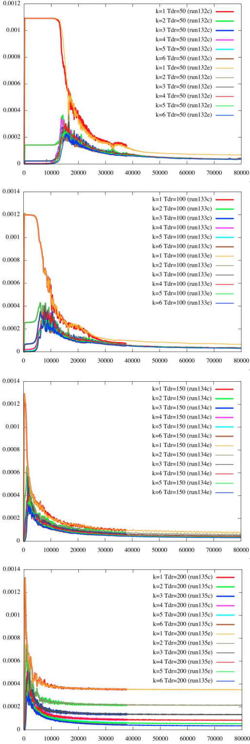
Fig. 23. Time evolution of \sqrt{\int_{\mathbb{R}} |\hat{f}^{(k)}(t, v)|^2 dv} for k = 1, 2, \dots, 6 and for drive time 50, 100, 150, 200 (run132c-135c and run132e-135e) Parameters are \Delta t = 0.5 , non-uniform, 6-th order time scheme and (N_x, N_v) = (4096, 32768) for run132c-135c, (N_x, N_v) = (2048, 16384) for run132e-135e.
