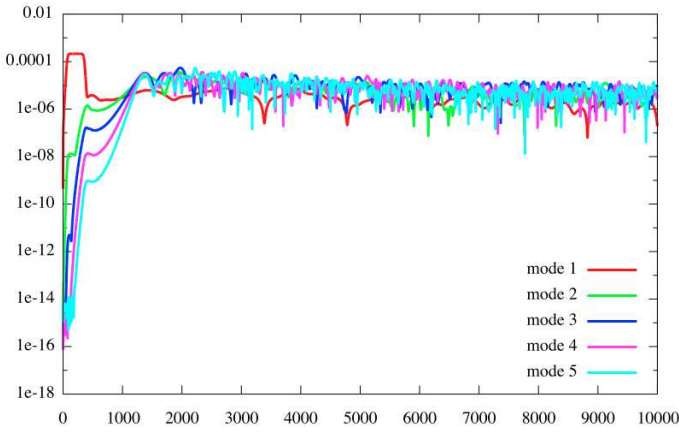
Fig. 13. a_{\text{dr}} = 0.00625 and T_{\text{dr}} = 150
