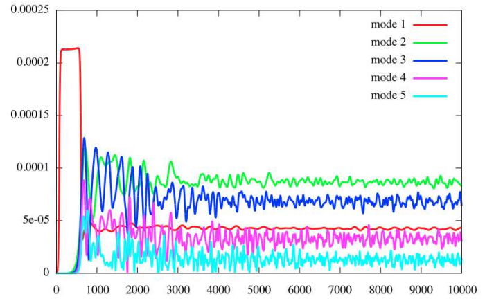
Fig. 18. a_{\text{dr}} = 0.00625 and T_{\text{dr}} = 400
