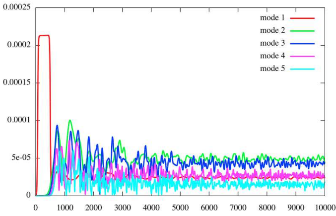
Fig. 17. a_{\text{dr}} = 0.00625 and T_{\text{dr}} = 300
