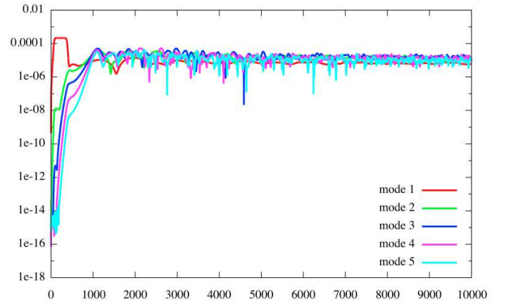
Fig. 14. a_{\text{dr}} = 0.00625 and T_{\text{dr}} = 175
