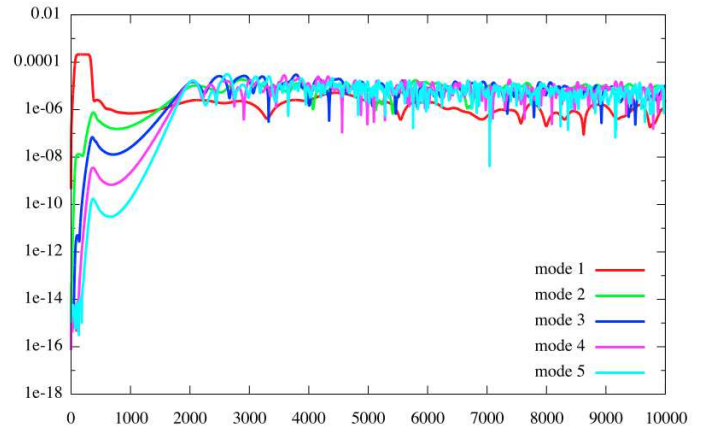
Fig. 12. a_{\text{dr}} = 0.00625 and T_{\text{dr}} = 125
