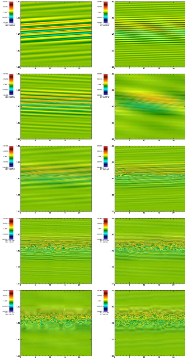
2048x16384x20000x11 dt=0.5 32nu a_drive=0.00625 tflat 100
