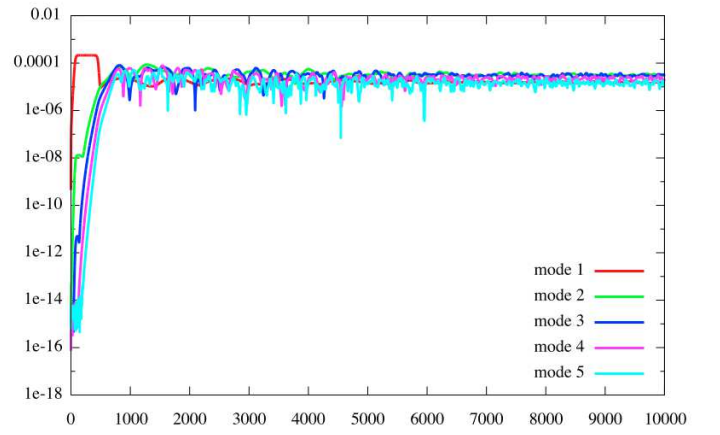
Fig. 16. a_{\text{dr}} = 0.00625 and T_{\text{dr}} = 250
