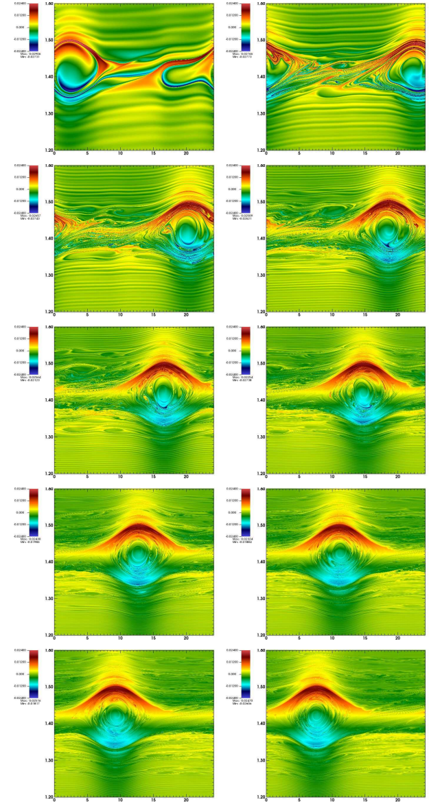
2048x16384x20000x11 dt=0.5 32nu a_drive=0.00625 tflat 400
