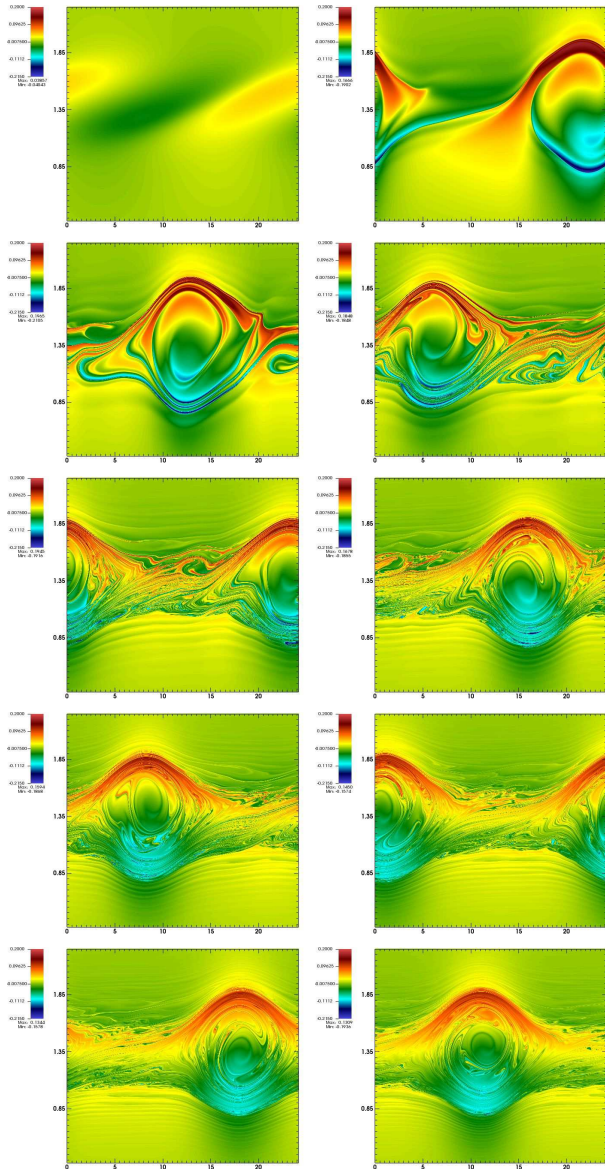
2048x16384x16000x11 dt=0.00625 32nu a_drive=0.2 11h hydra
