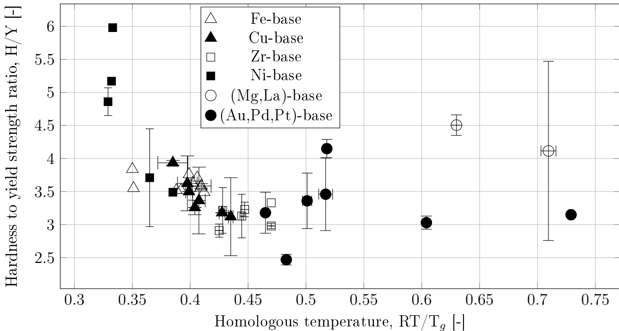
Fig. 1. Hardness-to-yield strength ratio as a function of reduced temperature RT/T_g for all metallic glasses ( RT refers to room temperature)
