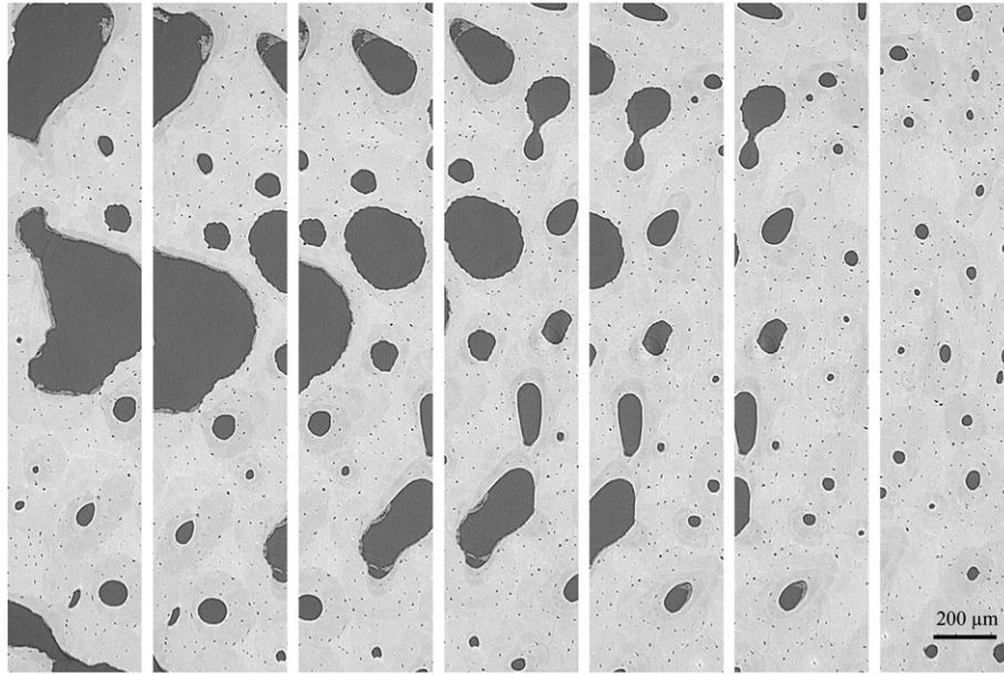
Fig. 7. A series of regions with different tissue porosities from a single sample. ((a)–(g): BV/TV ranging from 67% to 97%).
