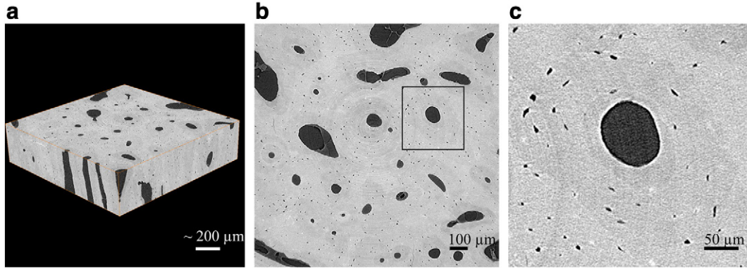
Fig. 1. (a) A 3D rendering of the reconstructed image ( 1000 \times 1000 \times 251 pixels). (b) A slice of reconstructed image from SR-CT with voxel resolution of 1.4 \mu\text{m} (image size: 1000 \times 1000 pixels). (c) Zoom around a Haversian canal.
