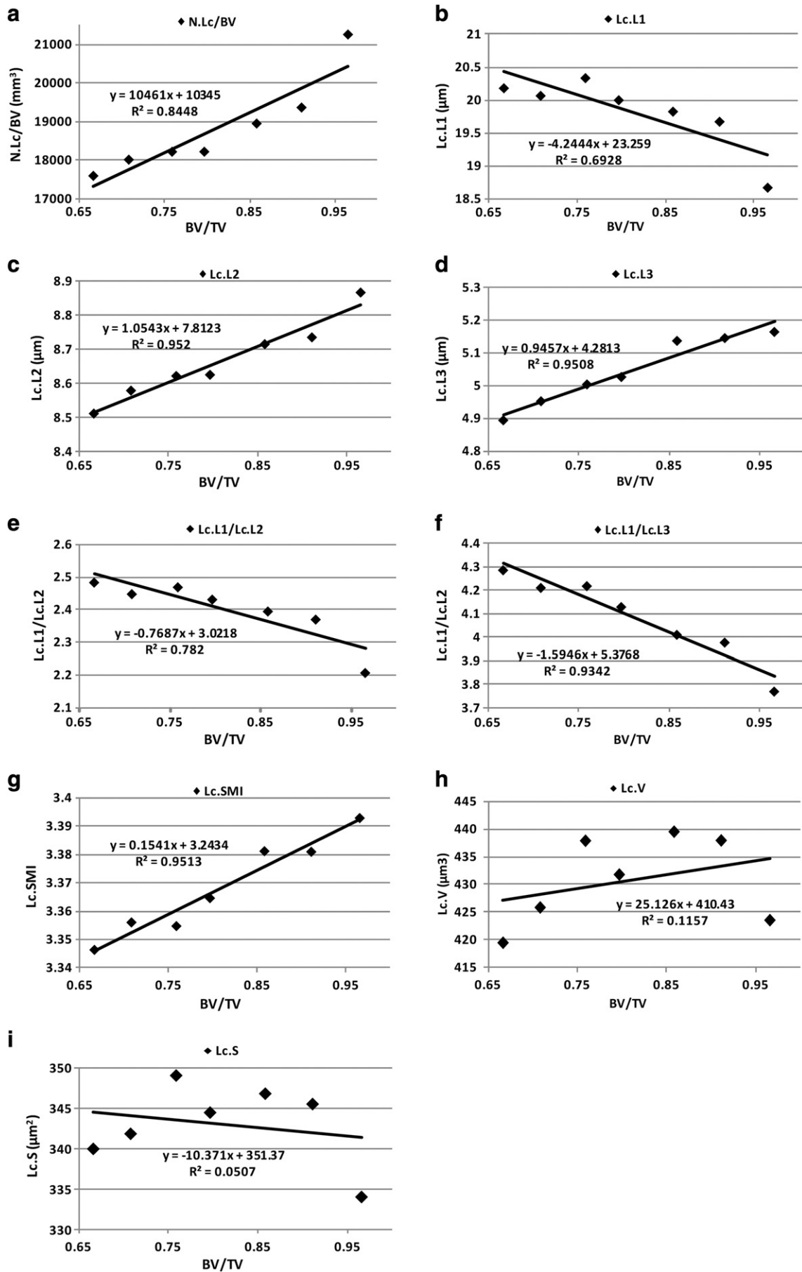
Fig. 8. Correlation of bone porosity with osteocyte lacunar density (a), axes lengths (b)–(d), anisotropy (e)–(f), SMI (g), volume (h) and surface area (i).
