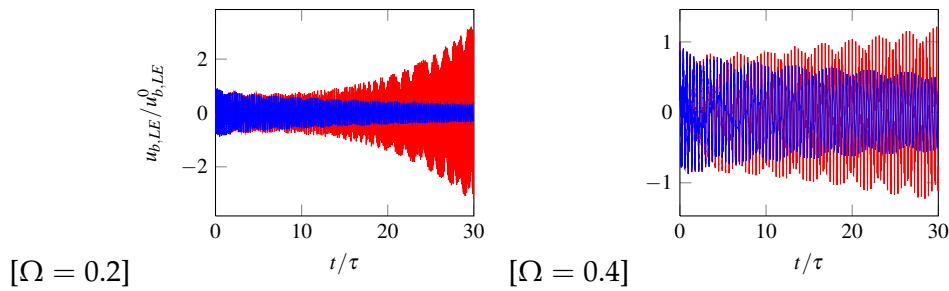
Figure 7: Tip radial displacement; K_e = 2 \cdot 10^3 N/m (—) and K_e = 2 \cdot 10^4 N/m (—)
