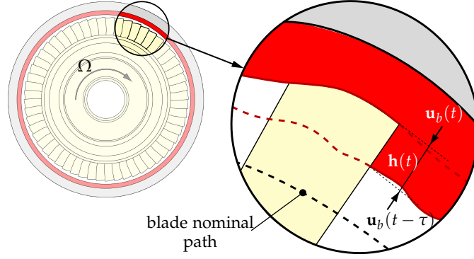
Figure 5: Schematic of abradsable material removal
