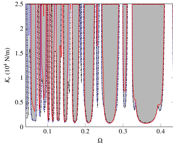
Figure 8: Time convergence: N = 40 (—); N = 60 (---), and N = 80 (-.-)
