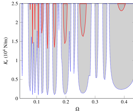
Figure 11: Instability lobes versus blade-tip contact location: trailing edge (—) and leading edge (- - -)
