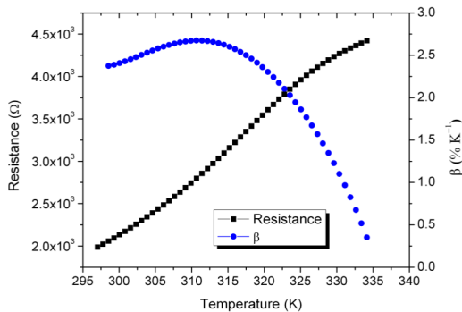
Figure 2. Sample's electrical resistance and \beta versus temperature
