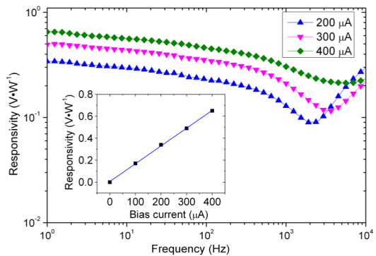
Figure 4. Optical responsivity versus laser modulation frequency at different bias currents at 318 K. The inset shows optical responsivity versus bias current at 1 Hz and 318 K.
