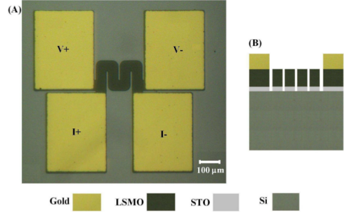
Figure 1. (A) Optical photograph of the tested sample with the two current probes [I+, I-] and two voltage probes [V+, V-]. (B) Schematic cross-section of the sample.
