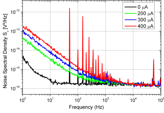
Figure 5. Noise spectral density measured in the four probe configuration at different bias currents at 318K.
