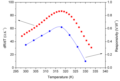
Figure 3. Optical responsivity \mathcal{R}_v at bias current 400 \text{ } \mu\text{A} and frequency 1 Hz and dR/dT versus temperature curves.
