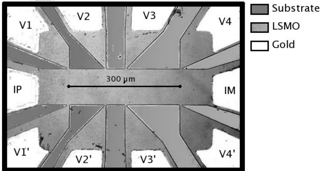
Fig. 4. Optical photograph of a 100 \mu\text{m} width line with the two current probes IP and IM and 4 voltage probes (V1...V4, V1'...V4') on each side of the line. The line lengths between V1 -V2, V2 - V3 and V3 -V4 are 100 \mu\text{m} , 50 \mu\text{m} and 150 \mu\text{m} , respectively.
