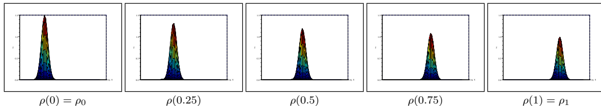
FIG 3. Plot of the isolevels of the density \rho(t) along the optimal path between two densities of different mass.
