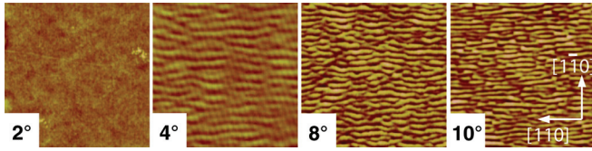
FIG. 1. (Color online) 1 \times 1 \mu\text{m}^2 AFM images of the LSMO films grown onto 2^\circ , 4^\circ , 8^\circ , and 10^\circ miscut STO substrates. Clear elongated structures on the top surface, oriented along the [110] crystallographic direction, are found in 4^\circ , 8^\circ , and 10^\circ miscut samples. No clear structures are observed in the lowest miscut film, i.e., 2^\circ .
