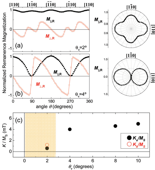
FIG. 3. (Color online) Angular dependence of the normalized remanence magnetization ( M_{\parallel,R}/M_S and M_{\perp,R}/M_S ) of 120-nm-thick LSMO films grown onto a vicinal (a) \theta_v = 2^\circ and (b) 4^\circ STO(001) surfaces. The right panels show the corresponding polar-plot representations of M_{\parallel,R} . Note that different scale is adopted for the 2^\circ miscut film. (c) Miscut angle \theta_v dependence of uniaxial anisotropy K_u (closed symbols) and biaxial anisotropy K_b (open symbols) constants. The shadowed area highlights the region of non-negligible biaxial anisotropy.
