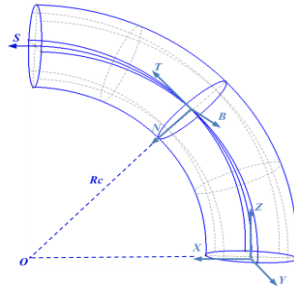
Figure 2. Schematic of an elbow with local curvilinear coordinates system
