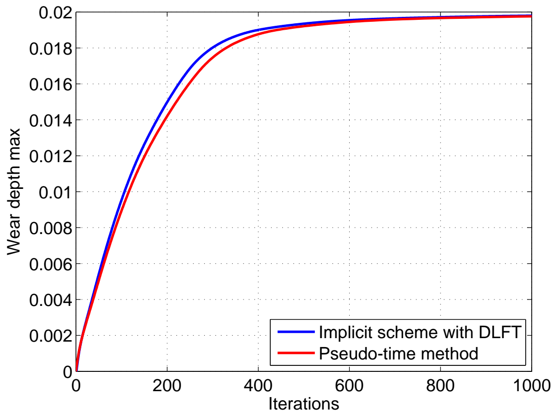
Fig. 11: Maximum wear depth evolution
