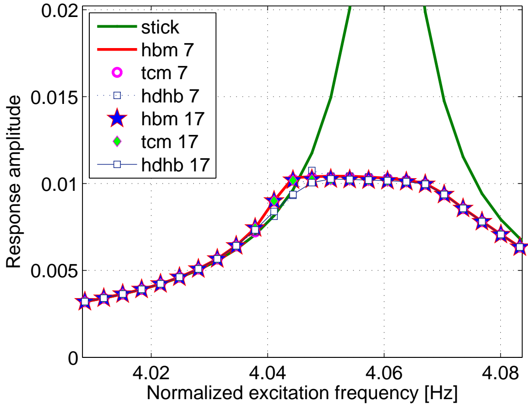
Fig. 5: Frequency response around first mode with different methods Nh = 7, 17
