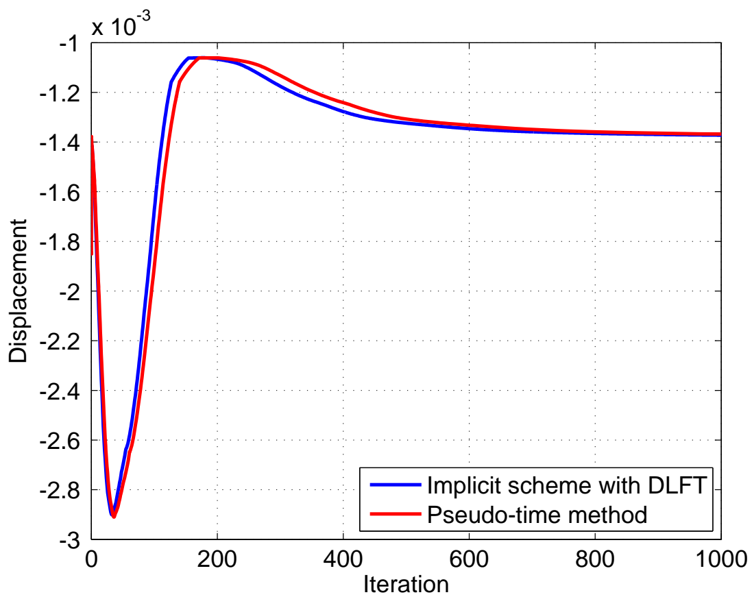
Fig. 12: Evolution of first harmonic value of tangential displacement for node 25
