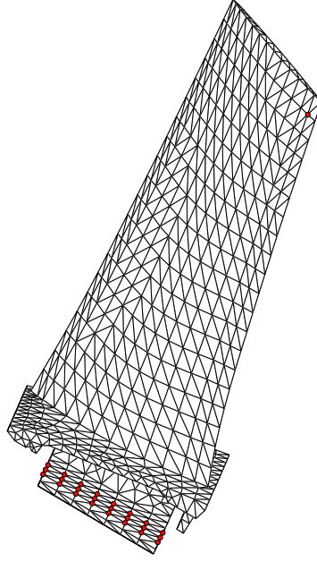
Fig. 2: Calculated bladed sector: finite element geometry
