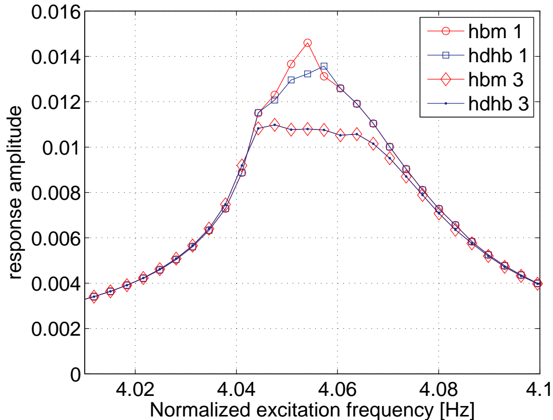
Fig. 6: Frequency response for HBM-1 with N_{it} = 2Nh + 1 and HDHB-1
