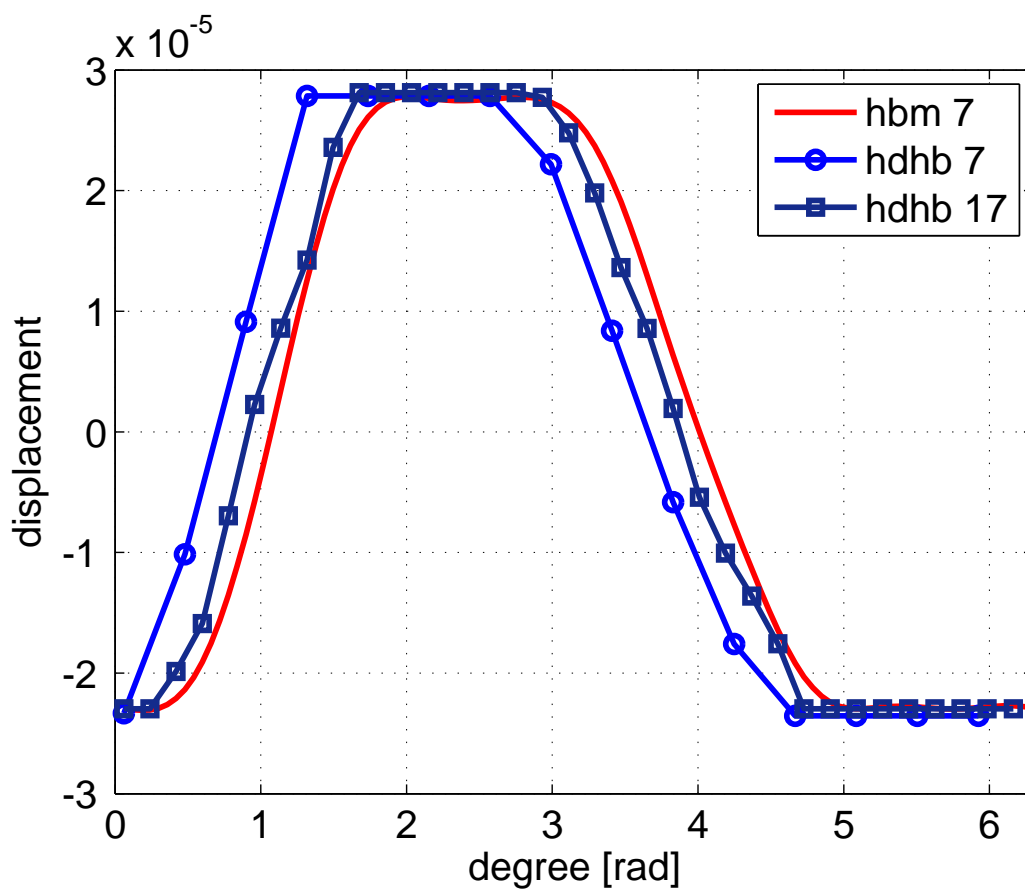
Fig. 8: Tangential displacement during one cycle
