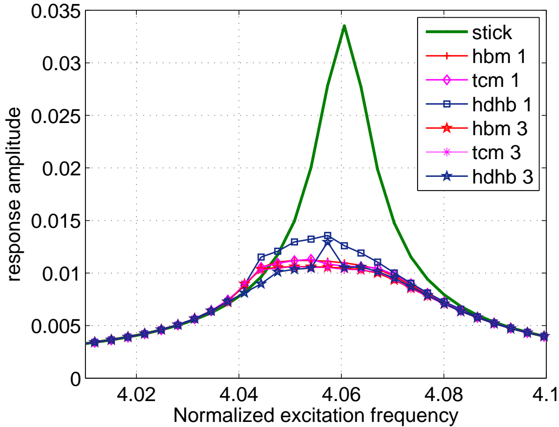
Fig. 4: Frequency response around first mode with different methods Nh = 1, 3
