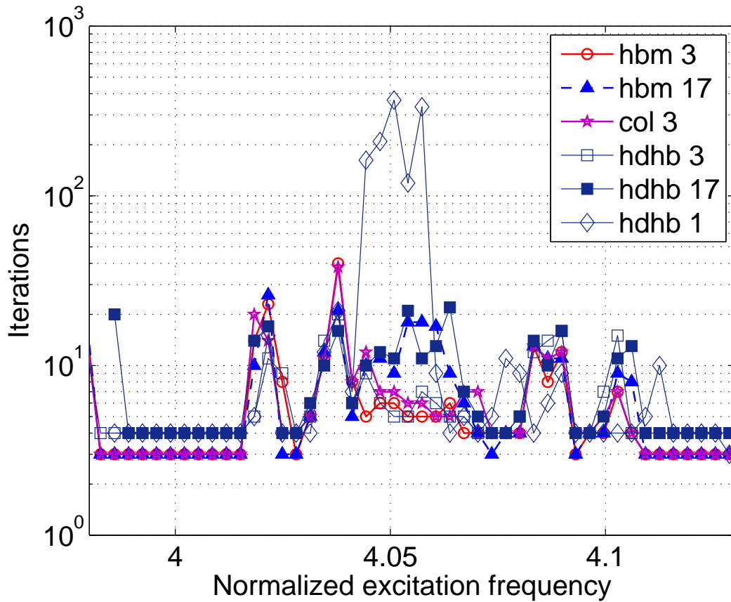
Fig. 7: Iterations versus frequency for different HB methods
