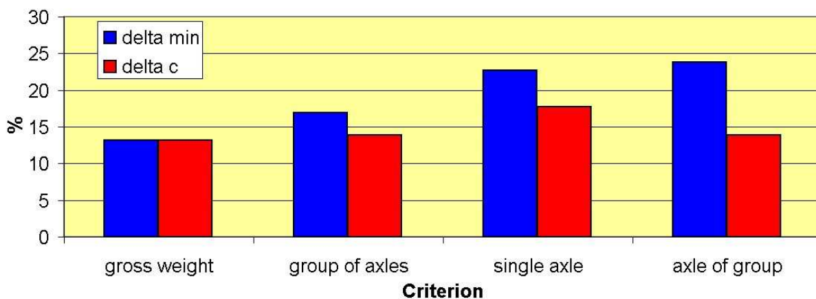
Figure 3: Classes of accuracy of this B-WIM test at the viaduct of Millau.
