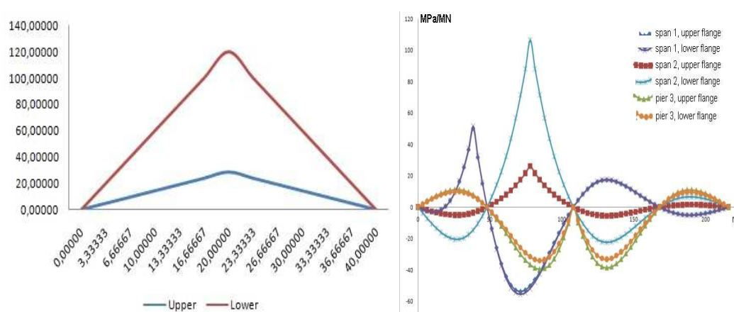
Figure 5: Influence lines that have been used in this study. On the left: influence line of the bending moment stress at mid-span of a simple supported 40 m span bridge, near Auxerre.
