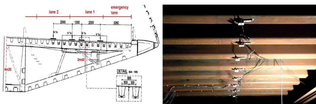
Figure 2: Millau viaduct. On the left: scheme of the box-girder. On the right: picture of the extensometers that have been glued to the bottom of the longitudinal stiffeners at mid-span of the first span.
