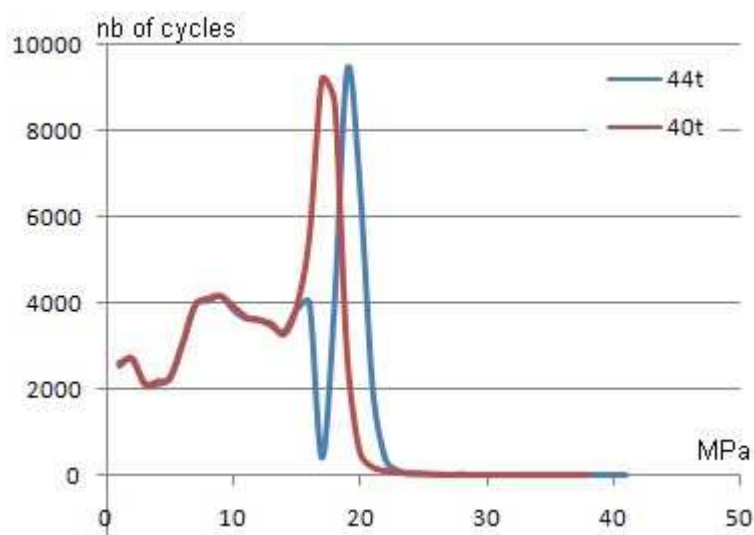
Figure 6: rain-flow histograms of the bending moment stresses in the lower flange at mid-span for both traffics (40 tons and 44 tons) on Auxerre bridge.
