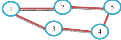
Figure 4 (a) : Undirected network
