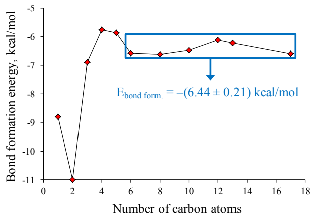
Figure 4. Reaction energies of bond formation reactions between the quartz surface and organic molecules containing a carboxylate group as a function of increasing side chains. The last six values were averaged.
