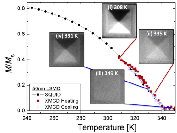
FIG. 2. (Color online) Scaled XMCD contrast vs temperature for a 50 nm LSMO square element, 3.3 \mu\text{m} size (full squares for heating and empty squares for cooling) and SQUID magnetometry measurements (circles), used to calibrate the temperature scale for the XMCD data. The inset shows XMCD images of the domain states at (1) 308 K, (2) 335 K, (3) 349 K, and (4) 331 K in the cooling cycle.
