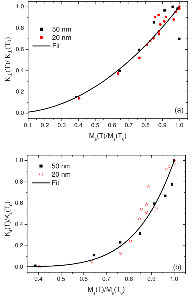
FIG. 10. (Color online) (a) Normalized perpendicular uniaxial anisotropy coefficient k_{\perp} = K_{\perp}(T)/K_{\perp}(T_0=4 \text{ K}) and (b) normalized in-plane fourfold anisotropy coefficient k_4 = K_4(T)/K_4(T_0=4 \text{ K}) as a function of the normalized magnetization m = M_s(T)/M_s(T_0=4 \text{ K}) for the 20-nm-thick and 50-nm-thick samples.
