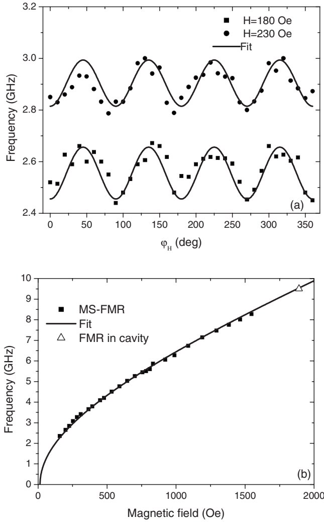
FIG. 5. (a) MS-FMR in-plane angular dependence of the resonance frequency. (b) Resonance frequency of the uniform mode as a function of the in-plane applied field (parallel to the x axis) in the \text{La}_{0.7}\text{Sr}_{0.3}\text{MnO}_3 (50 nm)/ \text{SrTiO}_3 (20 nm)/Si sample.
