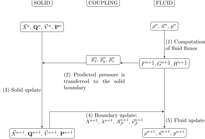
Figure 4: Structure of the coupling scheme
