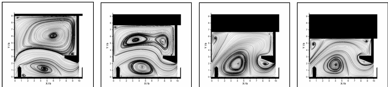
Fig. 2 - Streamlines and velocity in a vertical slot fishway: I = 10\% , B/b = 9, 7.66, 6.66 and 5.66 , Q = 23 L/s at Z/b = 2
