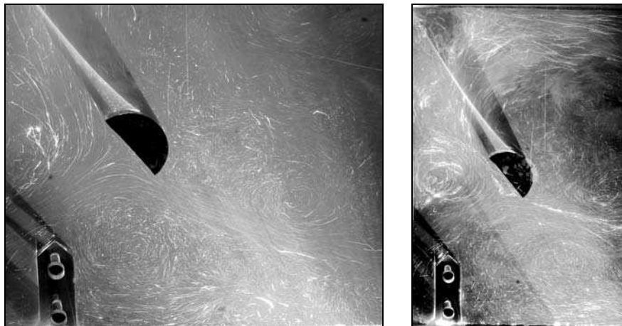
Fig. 8 - Flow visualizations in a fishway with a half-cylinder (plane face directed towards the flow): I = 10\% , B/b = 9 and 6.66 , Q = 23 L/s at Z/b = 0.26
