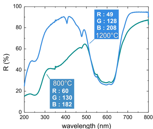
Fig. 6. Diffuse reflectance spectra ( R\% ) of \text{Zn}_{0.9}\text{Co}_{0.1}\text{Al}_{2.2}\text{O}_4 compound prepared at 800^\circ\text{C} (a) and 1200^\circ\text{C} (b).
