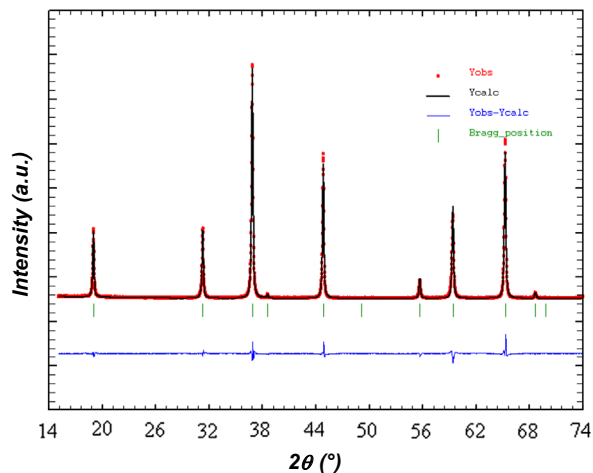
Fig. 10. Rietveld refinement spectra (experimental, calculated and difference) of \text{Mg}_{0.9}\text{Ni}_{0.1}\text{Al}_2\text{O}_4 composition annealed at 1200 °C.
