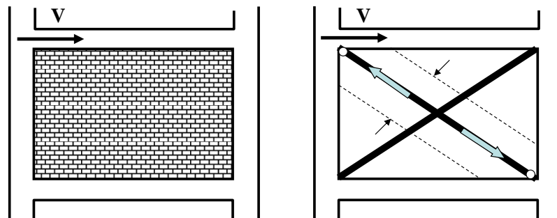
33 34 35 36 37 38 39 40 41 42 43 44 45 Fig. 2 Diagonal strut model 46 47 48 49 50 51
