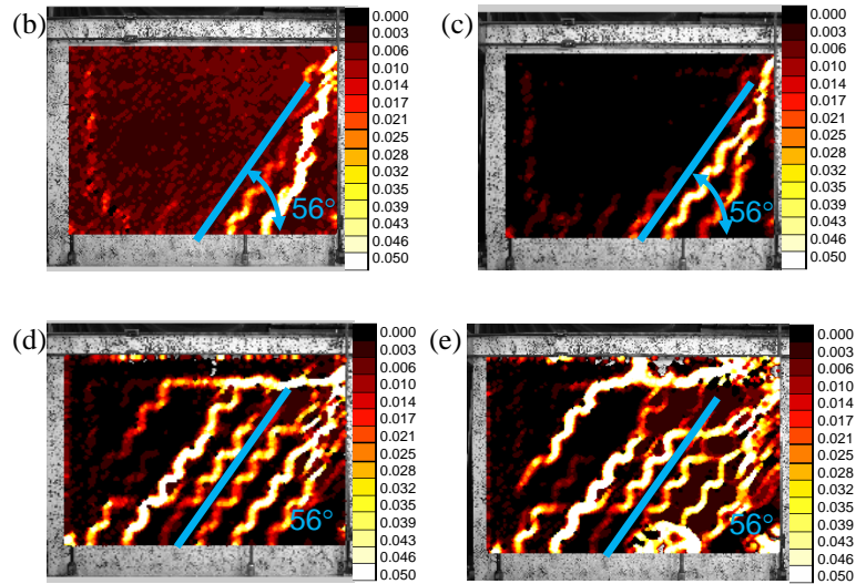
Fig. 15 Single bay infilled frame (IF2) (a) Force vs. stroke response; (b) and (c) Strain fields before the peak; (d) Strain field in the peak; (e) Strain field after the peak
