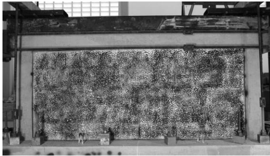
34 35 Fig. 12 Squat infilled frame (SF) 36
