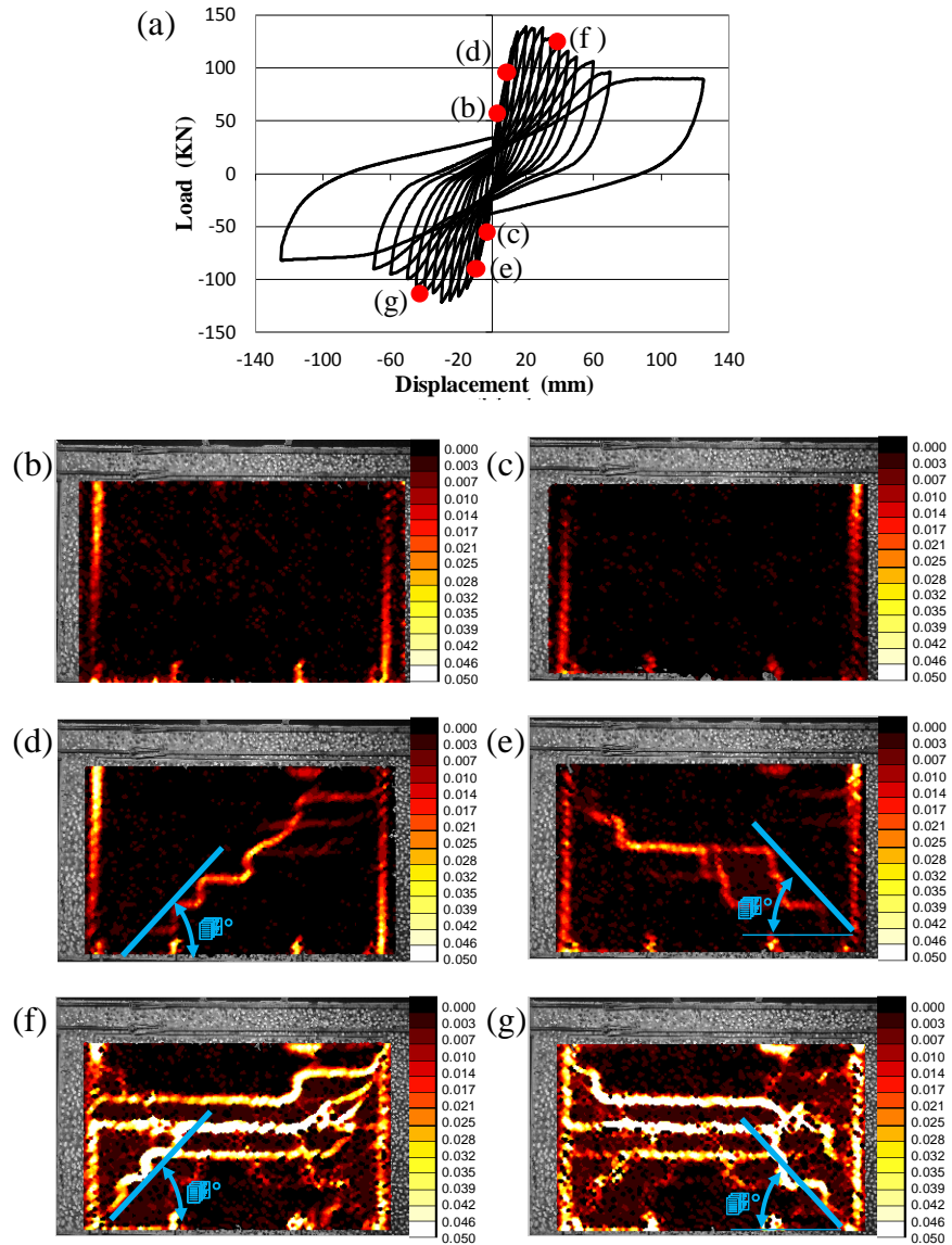
Fig. 7 Single bay infilled frame (IF1); (a) Force vs. displacement curve; (b) and (c) Strain fields in the first cycle; (d) and (e) Strain fields in the second cycle; (f) and (g) Strain fields in a subsequent cycle after the peak
