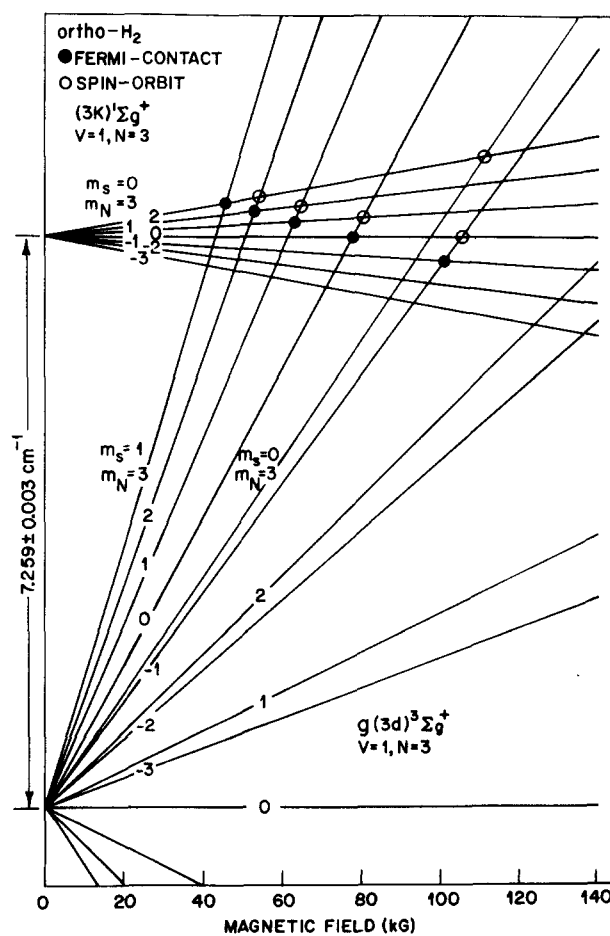
FIG. 2. Energy level diagram of the N=3 \leftrightarrow N=3 anti-crossings.
