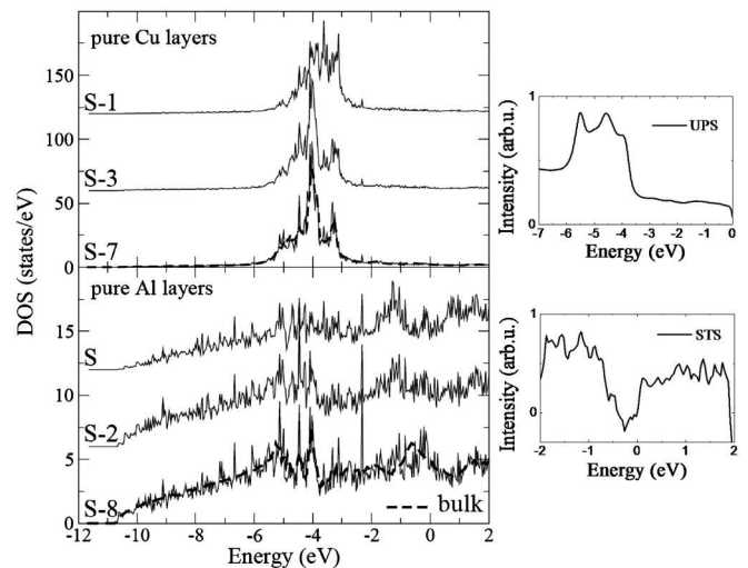
FIG. 4. DOS of the surface ( S ) and subsurface ( S-1, S-2, S-3, \dots ) layers. UPS valence-band spectrum of the clean surface up to 7 eV below the Fermi level. STS measurements on the clean Al 2 Cu(001) reconstructed surface. The normalized dI/dV spectrum represents an average over 10^4 I(V) curves before differentiation.
