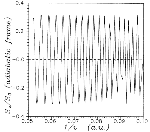
FIG. 9. Rosenthal oscillations in the polarization, after going through the outer crossing of Fig. 8. Purely classical simulation, with the coupling term included. The situation is formally similar to [20].
