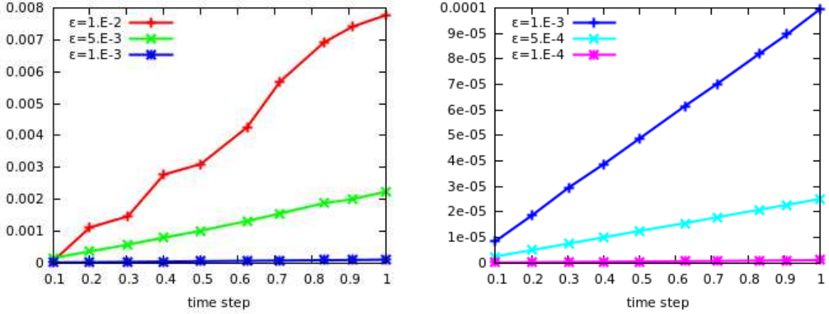
Figure 5: Maximum at time 10 of the mean of the Euclidean errors of the ETD-PIC method for several values of \varepsilon , obtained with the initial condition f_0 defined by (5.10)
