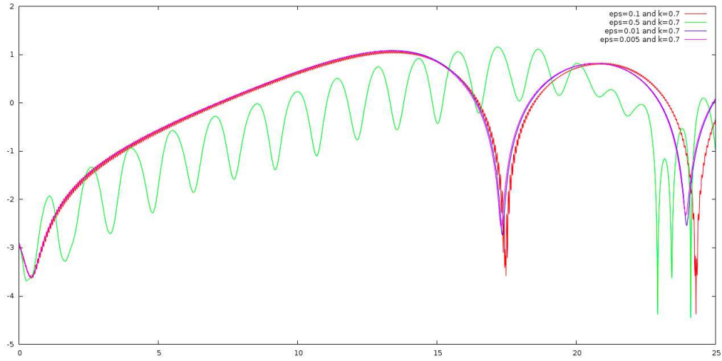
Figure 11: The growth rates for fixed k = 0.7 and several values of \epsilon from 0.5 to 0.005.
