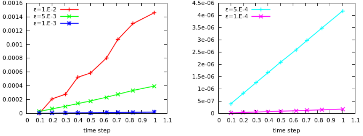
Figure 4: Global Euclidean errors of the ETD-PIC method at time 10 for several values of \varepsilon , obtained with an initial condition close to the slow manifold
