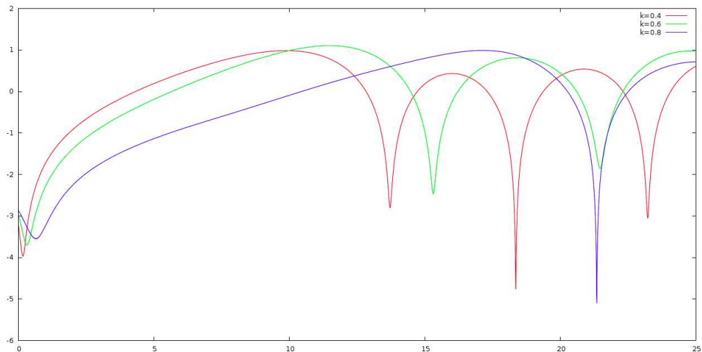
Figure 12: The growth rates for fixed \epsilon = 0.005 and three values of k .
