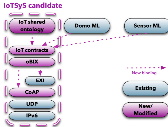
Fig. 3 Protocol stack for IoT building automation systems as proposed by [20]. Blocks that are introduced in this proposition or requiring some adaptations relative to their traditional use are presented in pink. Existing blocks requiring no adjustment are presented in blue. New bindings between blocks are shown with pink arrows.
