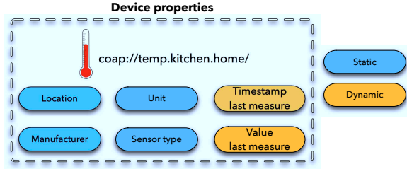
Fig. 1. Static and dynamic properties of a resource
