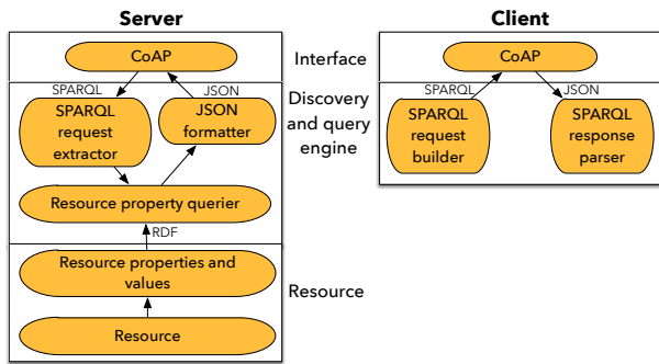
Fig. 3. Modules composing the client and server discovery architecture
