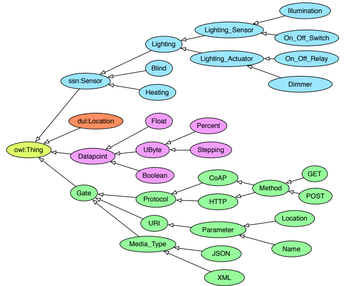
Fig. 2. Excerpt of the proposed ontology dedicated to building automation systems
