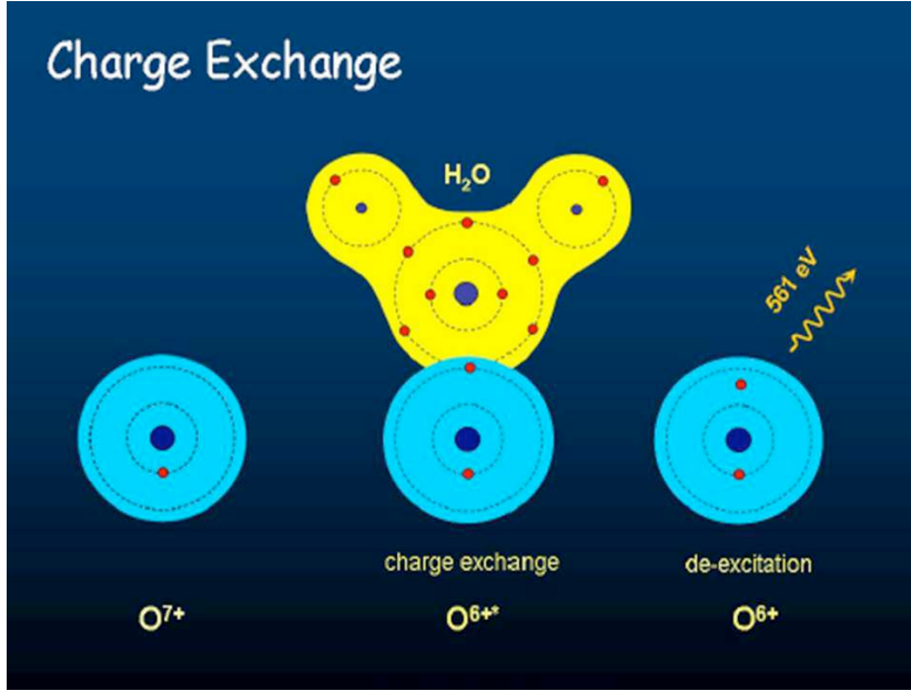
Fig. 23 Cartoon illustrating the CX process in the case of an \text{O}^{7+} ion from the solar wind encountering a water molecule of a cometary coma, acquiring an electron, being left in an excited state and emitting an X-ray line (from Dennerl (2009)).
