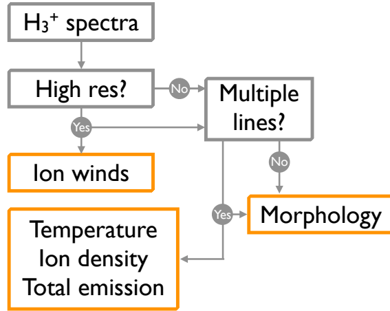
Fig. 18 A flowchart of the parameters that can be derived from \text{H}_3^+ spectral observations, which is a function of spectral resolution, wavelength coverage, and signal-to-noise.
