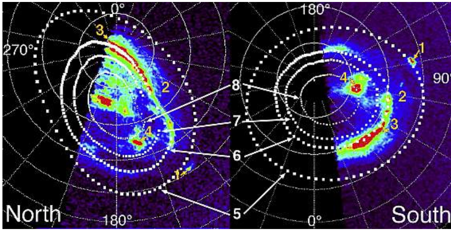
Fig. 33 Two consecutive color-coded polar projected maps of Jupiter’s aurora on 15 August 1999 using HST-STIS (1180–1530 Å FWHM). Dark blue: the faint solar reflected flux, light blue-green: moderate emissions including (2) the ‘low-latitude belt’, and red: brightest auroral features, (1) Io footprint, (3) main oval, (4) conjugate polar cusps. The dotted curve on top of (3) is the Pallier-Prangé (PP) reference main oval. (7, 8) are the PP derived inner reference ovals, and (5) is the VIP4 model Io footprint. From Pallier and Prangé (2004).
