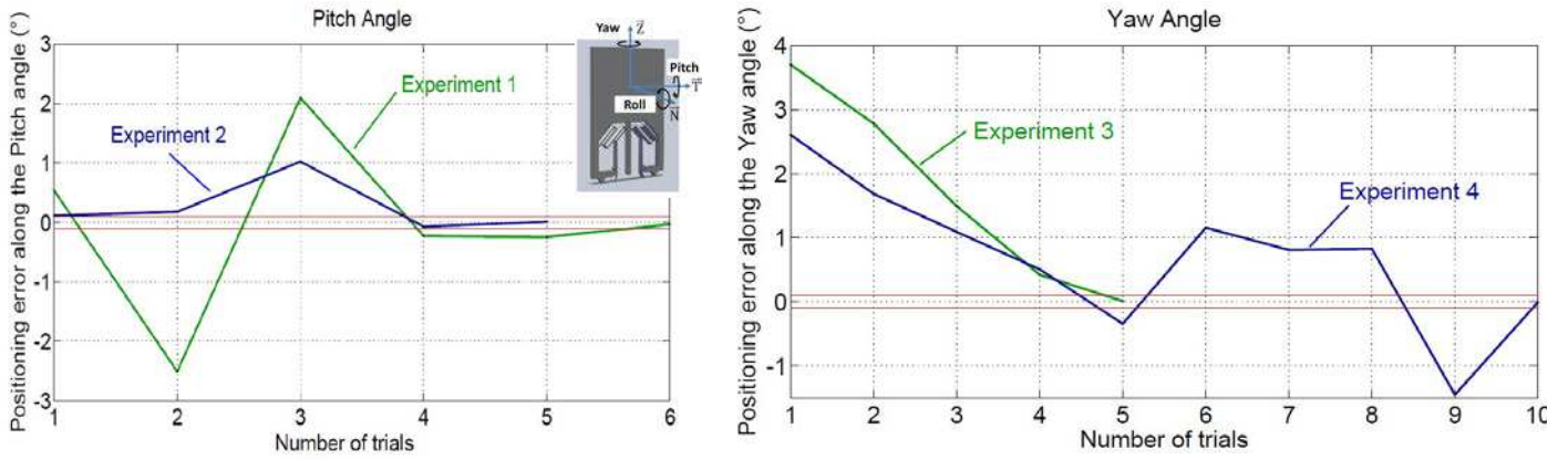
Fig. 5: Experimental results: (a) positioning error along the Pitch angle: experiment 1 requiring 6 trials to reach the target ( 0^\circ \pm 0.1^\circ ) and experiment 2 requiring 5 trials (b) positioning error along the Yaw angle: experiment 3 requiring 5 trials to reach the target ( 0^\circ \pm 0.1^\circ ) and experiment 4 requiring 10 trials.
