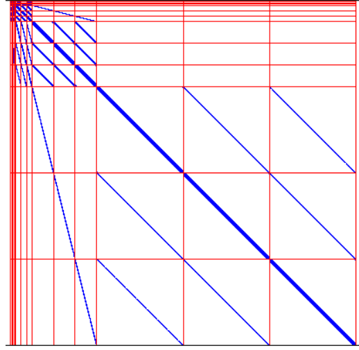
(b) Algorithm 2 – K = 30N^2
