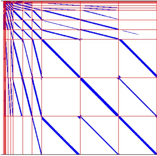
(c) Algorithm 1 – K = 128N^2
