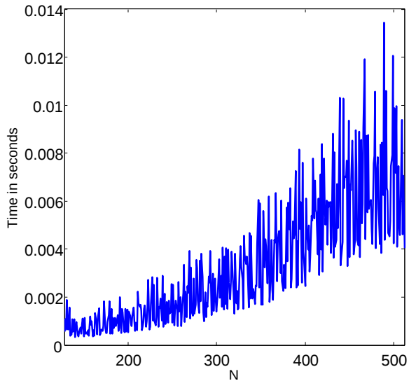
Figure 6: In this experiment, we evaluate the computing time of 2D FFTs applied to images of size N \times N . We use the FFTW in Matlab and do not include the time needed to compute the plans.
