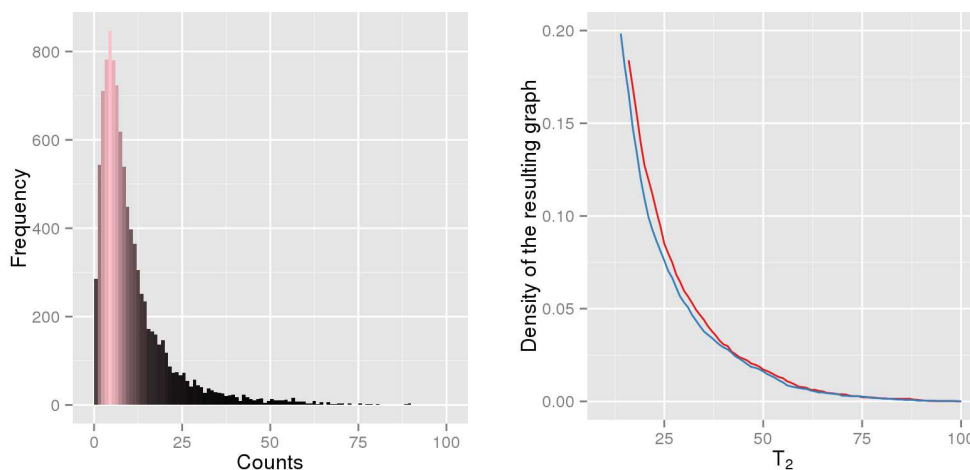
Figure 3: Distribution of the number of times an edge is selected over 100 bootstrap samples for the first condition (left) and Evolution of the density versus T_2 for the 2 conditions (right). T_1 = 500 , \mu = 1
