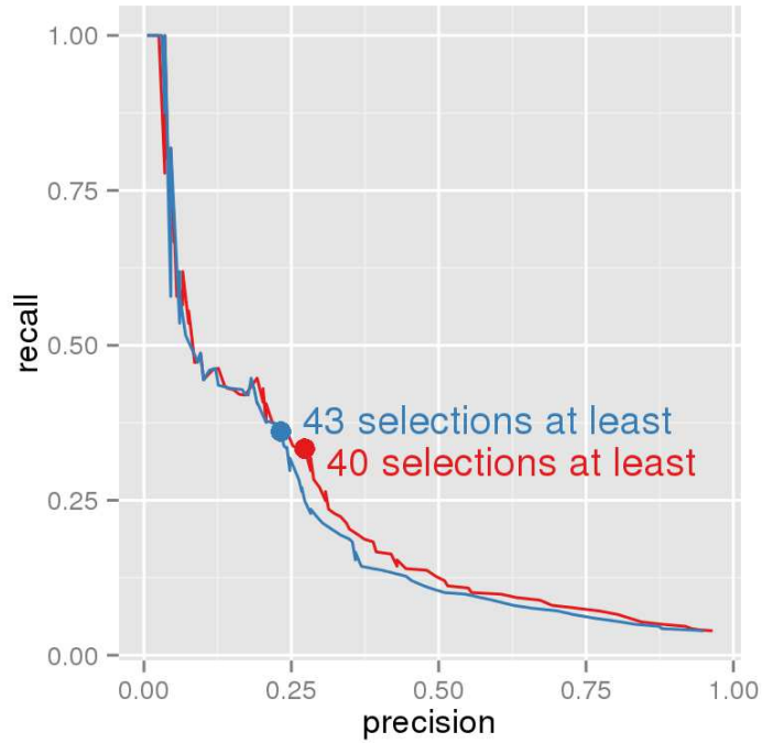
Figure 4: Precision/Recall curve (with varying T_2 ) for the total number of edges of the true child networks compared to the corresponding inferred network. T_1 = 500 , \mu = 1 (each curve correspond to one of the k = 2 child networks).
